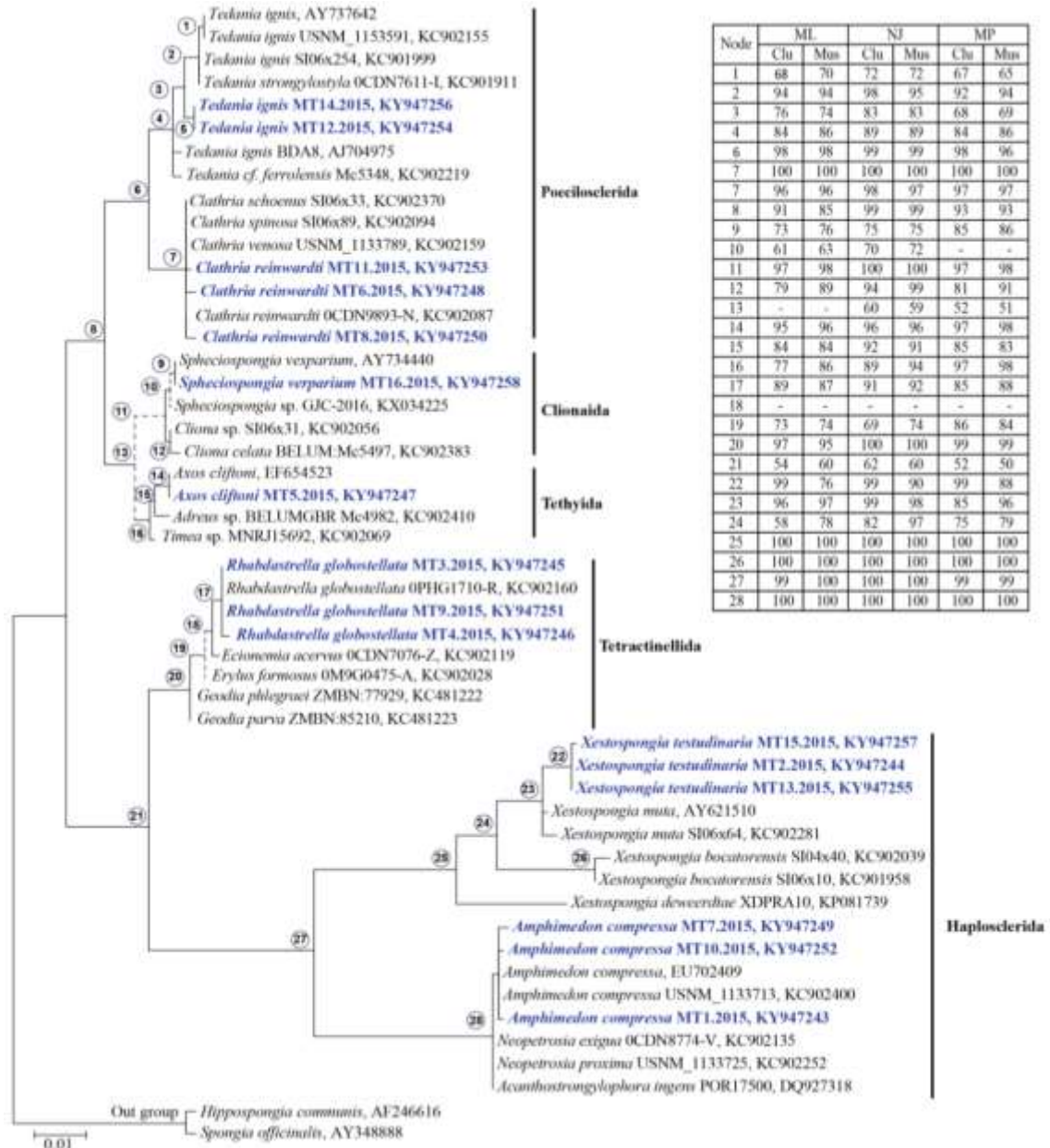
Figure 1. Phylogeny of 18S rRNA gene sequences of sponges in our study (blue bold letters) and from NCBI. The tree topology was obtained from NJ. Individual bootstrap values from ML, NJ, MP with alignment methods ClustalW (Clu) and Muscle (Mus) are located in the upper-right box and correspond to circled numbers on tree nodes. Solid lines indicate well-supported branches (support values greater than 50% for all criteria) and dashed lines indicate weakly supported branches
