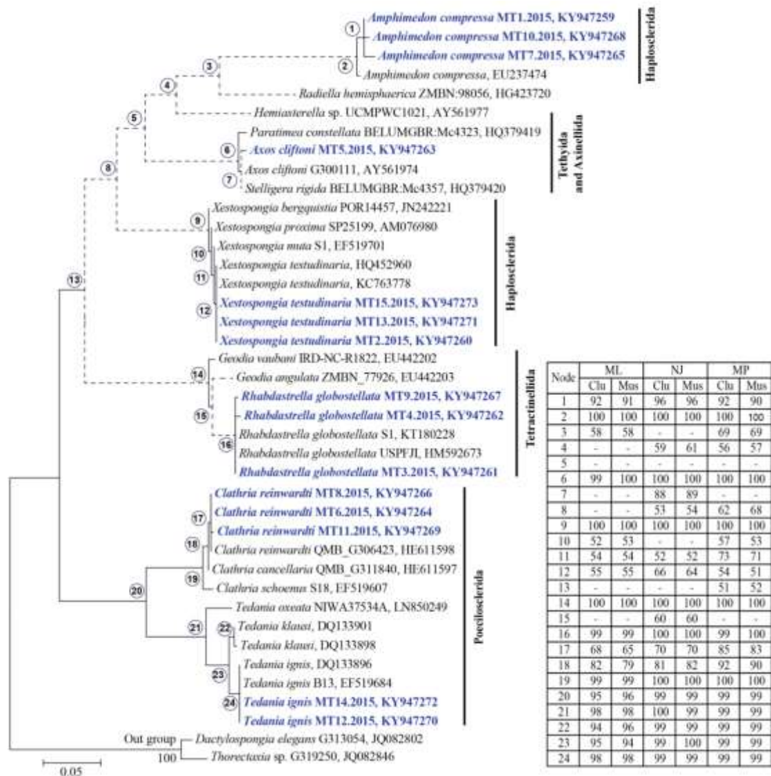
Figure 2. Phylogeny of partial COI gene sequences of sponges in our study (blue bold letters) and from NCBI. The tree topology was obtained from neighbor-joining (NJ) analysis. Individual bootstrap values from maximum likelihood (ML), NJ, maximum parsimony (MP) with alignment methods ClustalW (Clu) and Muscle (Mus) are located in the lower-right box and correspond to circled numbers on tree nodes. Solid lines indicate well-supported branches (support values greater than 50% for all criteria) and dashed lines indicate weakly supported branches.
